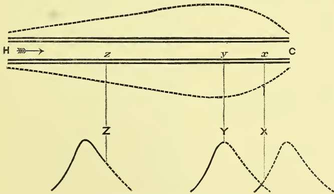
FIG. 46. A ROUGH DIAGRAMMATIC REPRESENTATION OF A PULSE WAVE PASSING OVER AN ARTERY.
